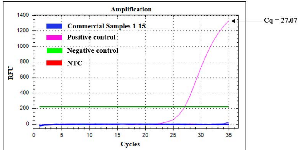
Figure 6. Real-time PCR amplification of DNA extracted from several meatball samples obtained from Yogyakarta, Indonesia.
