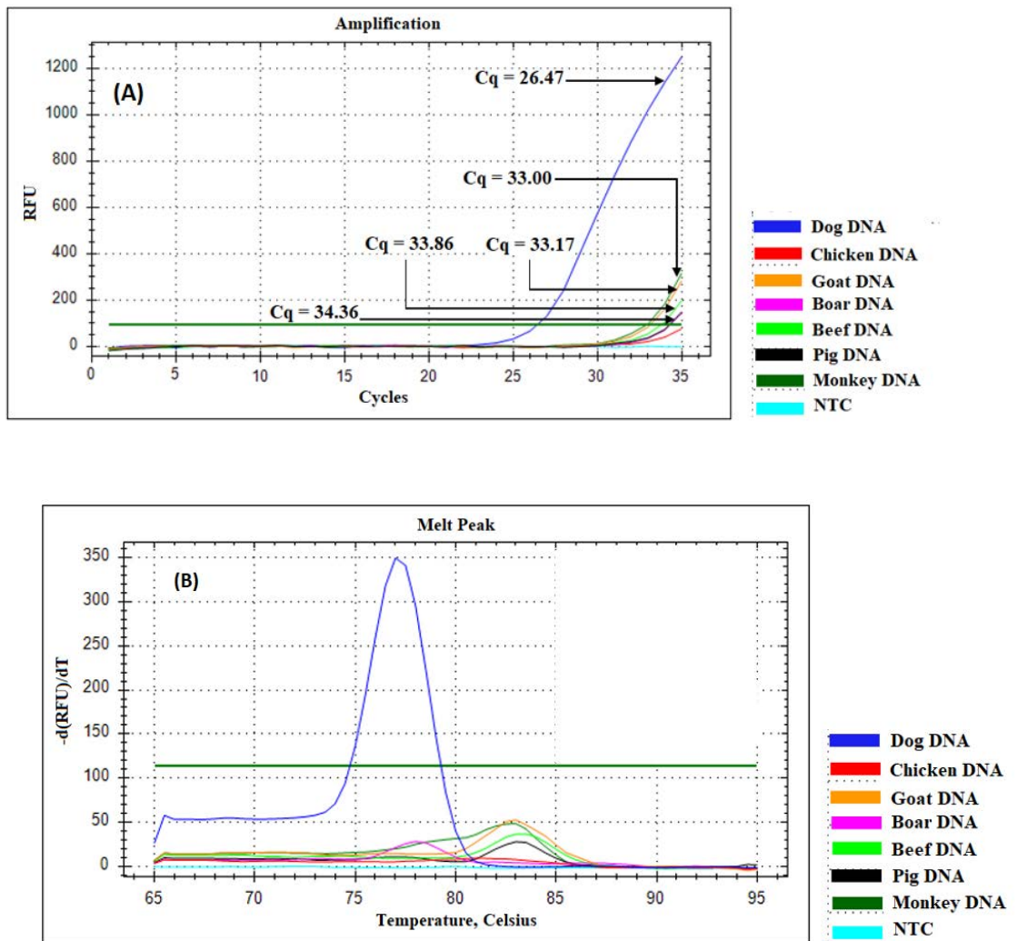
Figure 3. Specificity test of primer Cytb-55 towards DNA extracted from several meats using optimum annealing temperature of 57.9°C. (A) Amplification curve; (B) melting curve during amplification.
